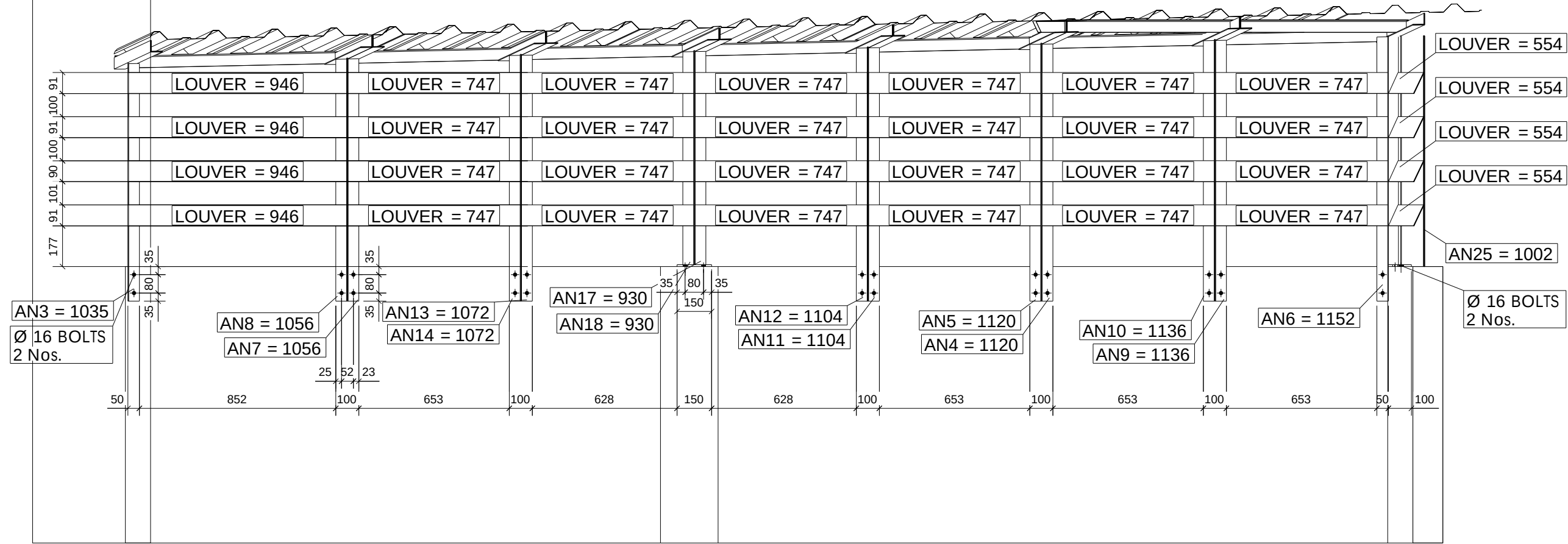
LOUVERS ELEVATION
